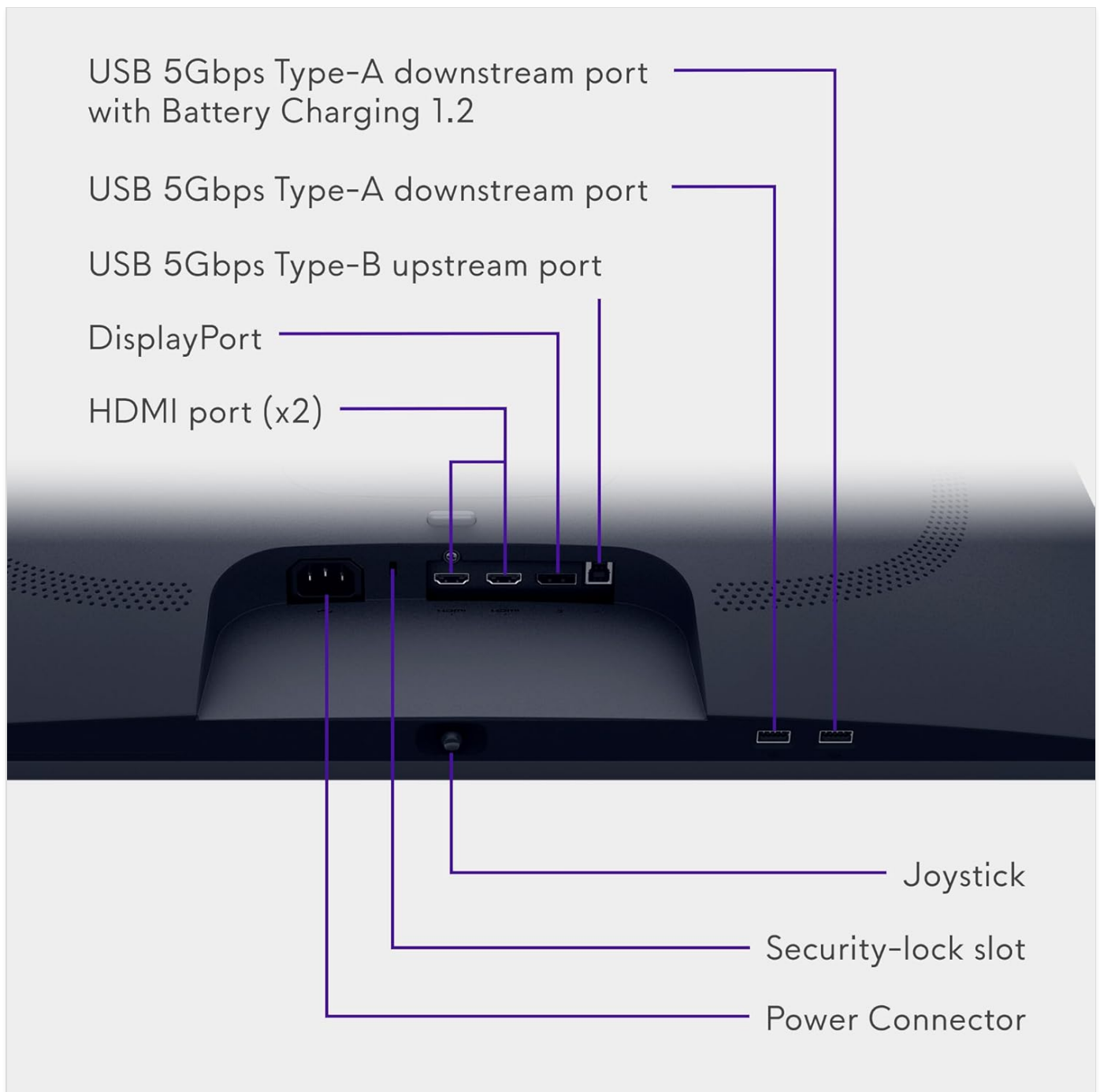
Figure 2.2: Diagram of monitor input/output ports including USB, DisplayPort, and HDMI.
