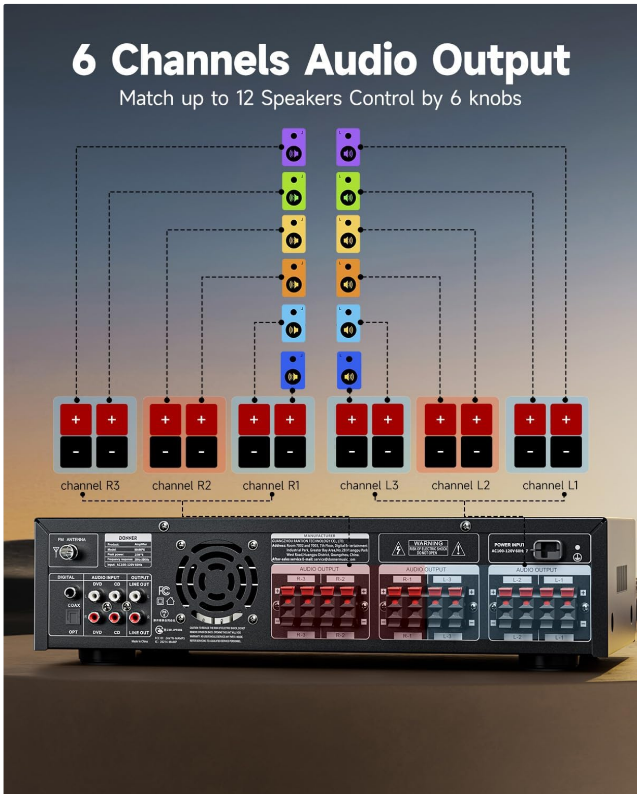
Image: A diagram illustrating the 6-channel audio output of the Donner MAMP6, showing how up to 12 speakers can be connected and controlled by individual volume knobs.
