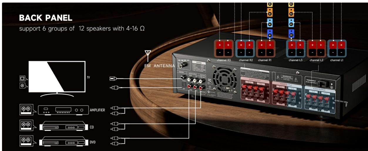
Image: A detailed diagram of the Donner MAMP6 back panel, showing connections for FM antenna, digital optical/coaxial, RCA inputs, line out, and the 6-channel speaker outputs.
