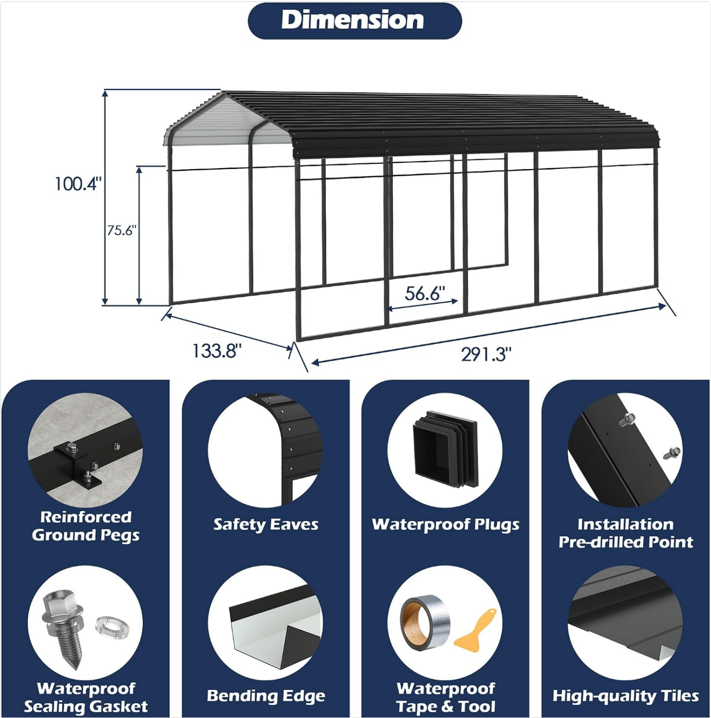
Figure 6: Carport dimensions and key features.
