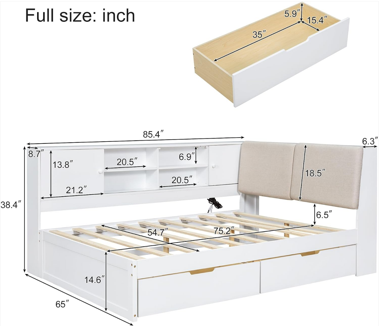
Detailed dimensions diagram for the Brabrety Full Size L-Shaped Daybed, including overall length (85.4"), width (65"), height (38.4"), and internal measurements for storage components.
