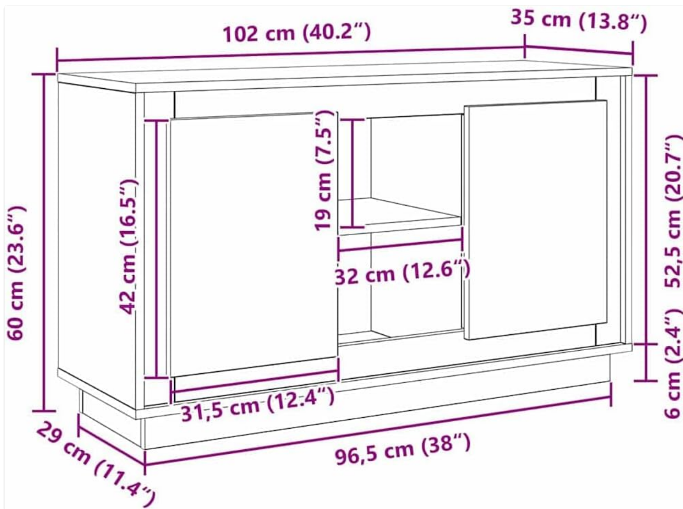
Image: Detailed dimension diagram of the sideboard, showing overall measurements and internal compartment sizes for assembly reference.
