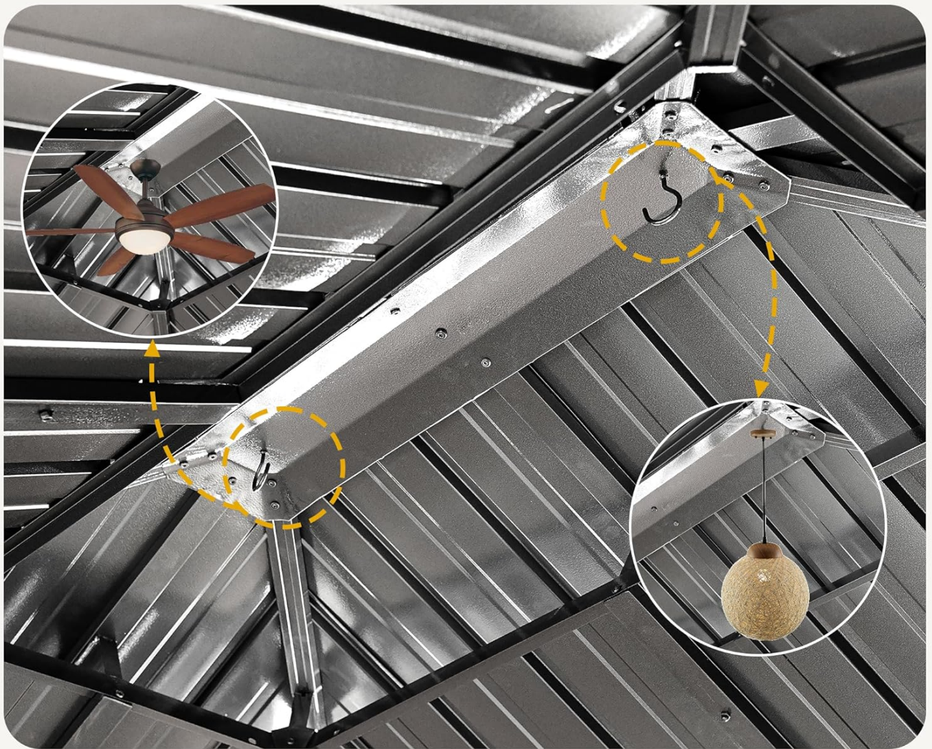
Image: Detail of the gazebo's roof structure, highlighting the integrated hooks designed for hanging accessories like lights or fans.
