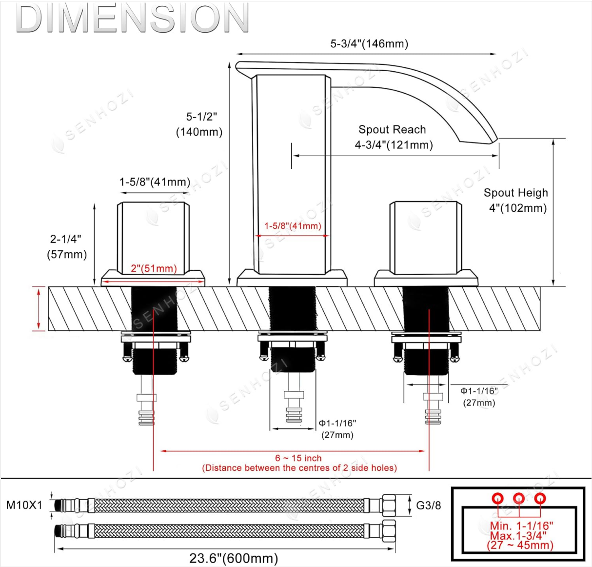
Image 3: Detailed dimension diagram for installation planning.
