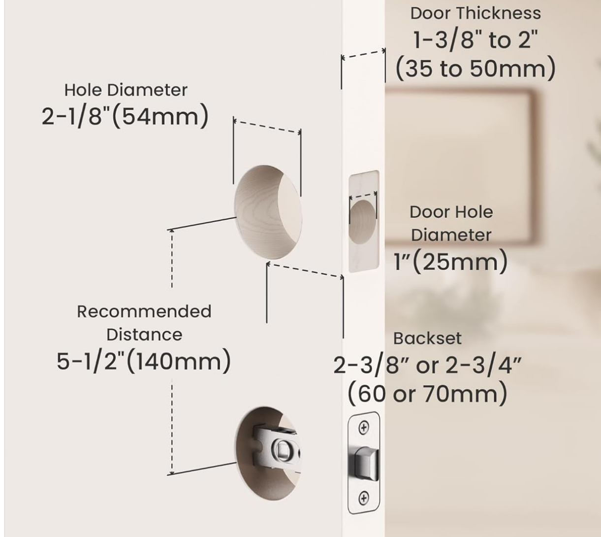
Figure 2: Door measurement guide for installation.
