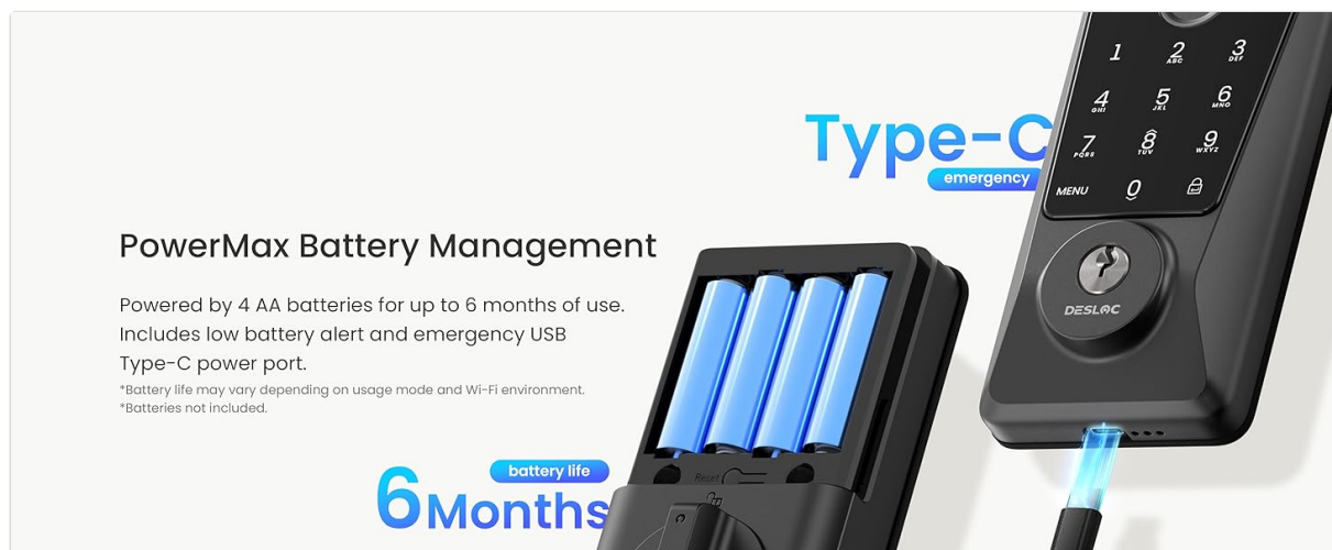
Figure 8: Battery installation and emergency power port.
