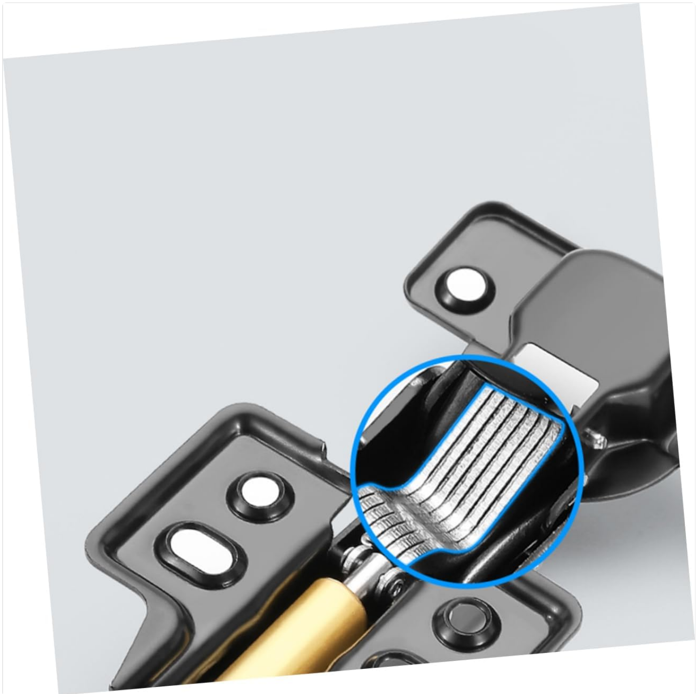
Image: An internal view of the hinge, showing the hydraulic pressure and damp buffer components responsible for its smooth and quiet operation.
