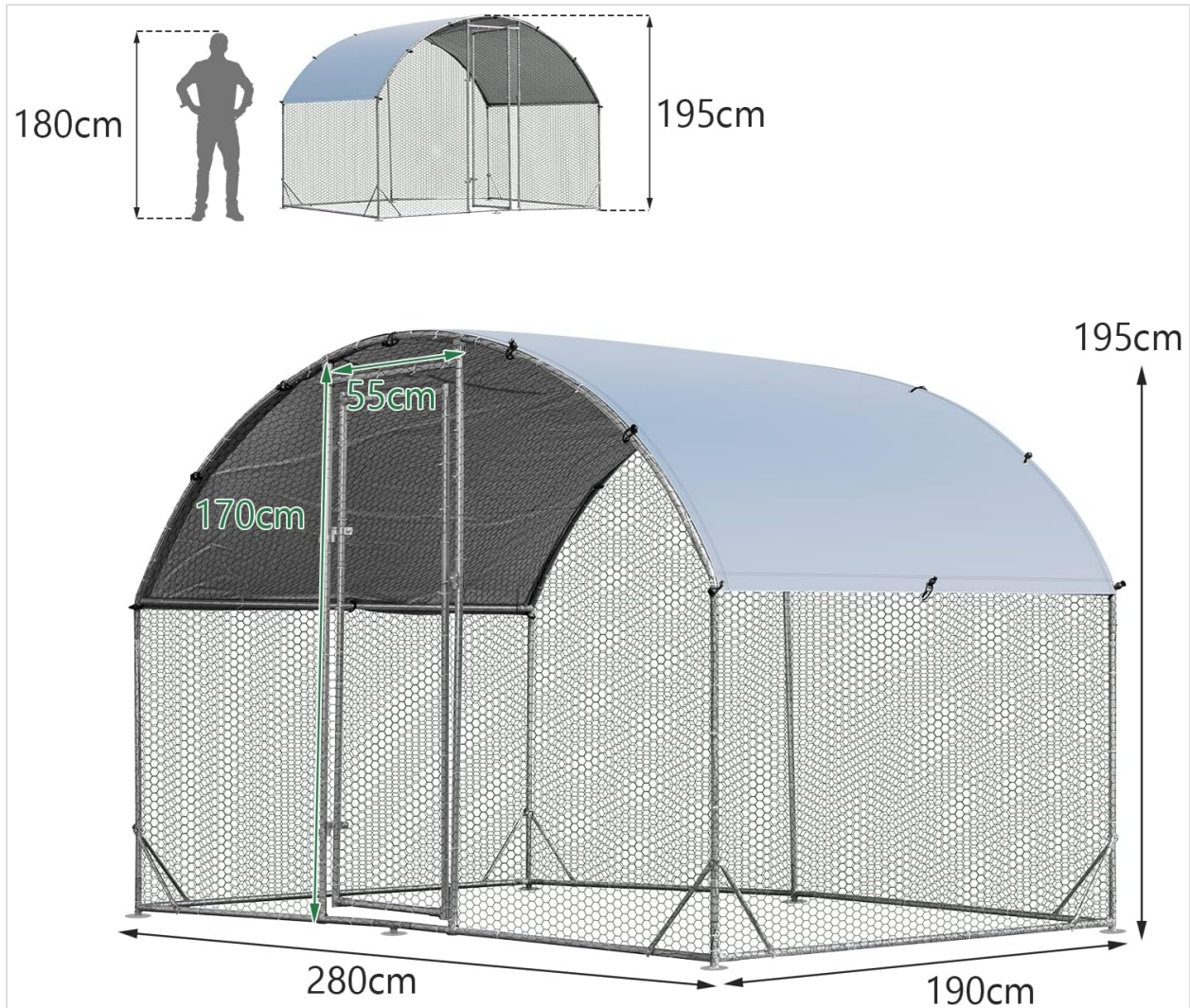
Image 7.1: Detailed dimensions of the poultry enclosure.
