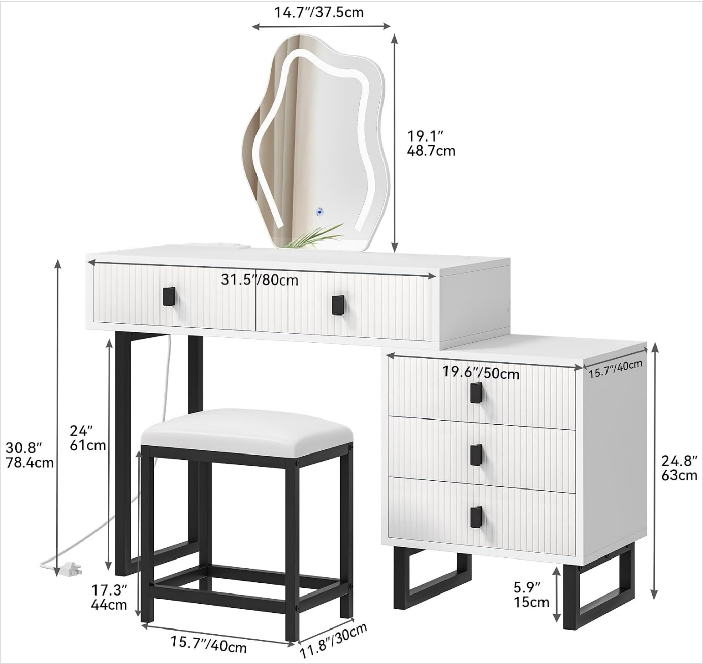
Figure 5: Detailed dimensions of the Moasis Makeup Vanity Set, including measurements for the mirror, desk, and side cabinet.
