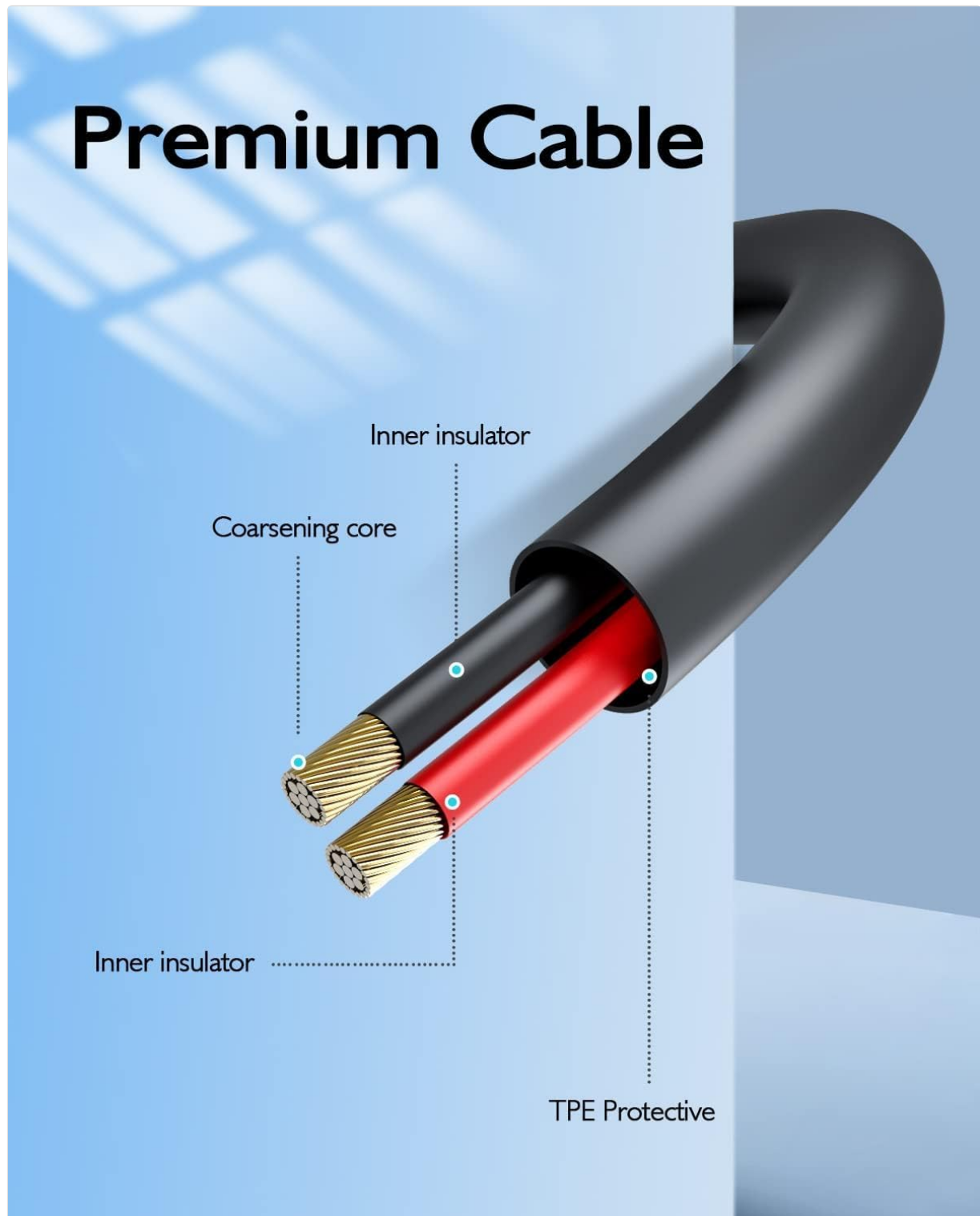
Image 5.1: The charger features a premium cable construction with an inner insulator, coarsening core, and TPE protective layer for durability and efficient power transfer.
