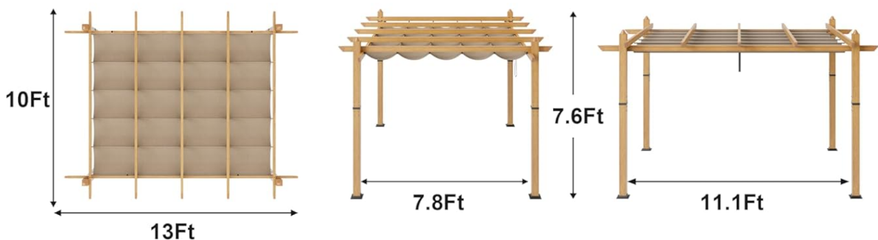
Image: Pergola Dimensions. This diagram illustrates the overall dimensions of the assembled pergola: 13 ft length, 10 ft width, and 7.6 ft height.
