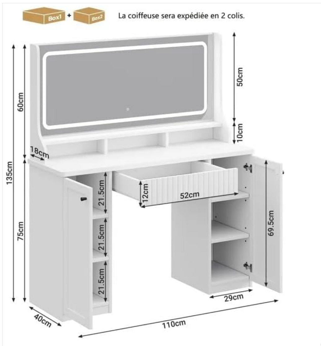
Figure 3: Dimensional diagram of the vanity table, illustrating key measurements and component placement for assembly reference.
