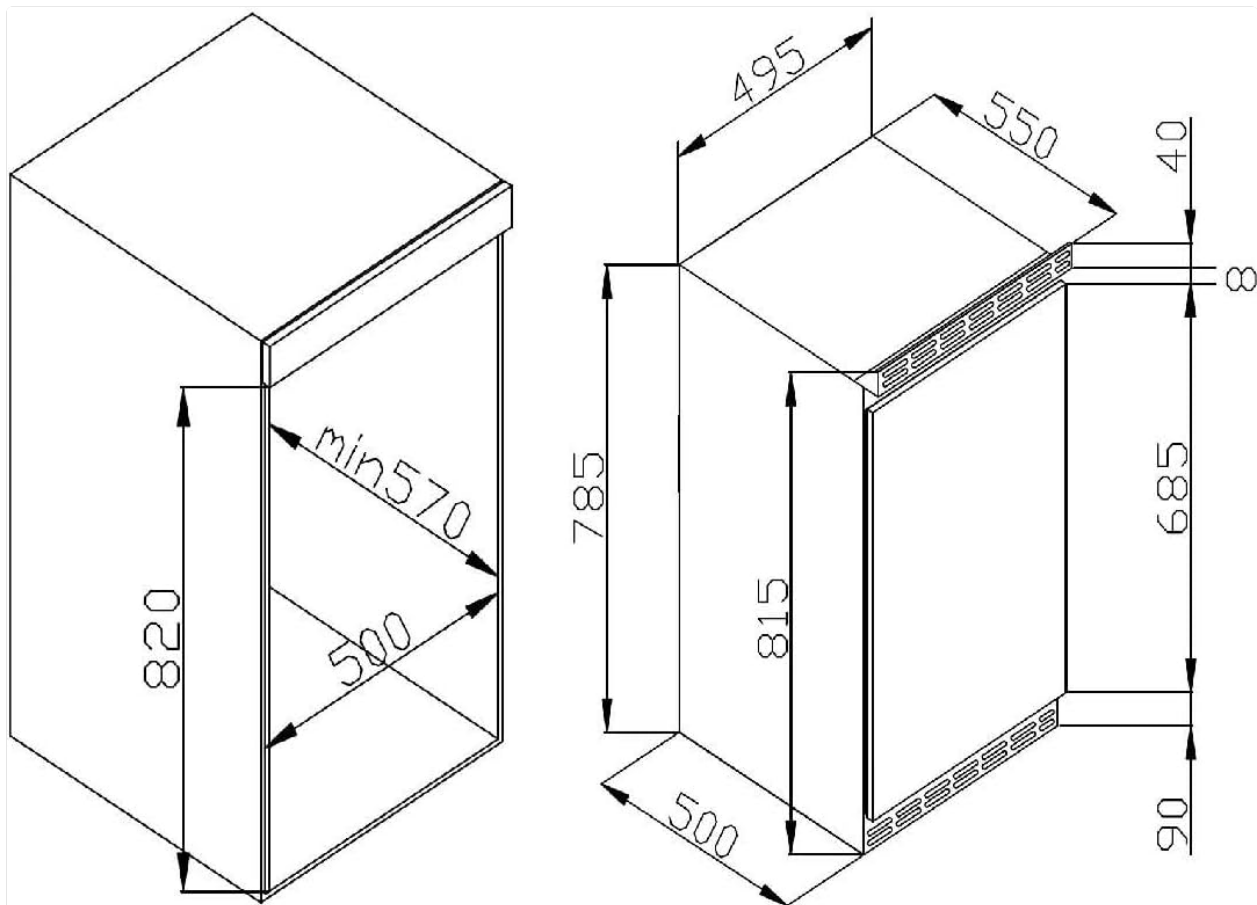
Image: Technical diagram illustrating the dimensions of the Amica UVKSD 351 961 refrigerator and the required built-in niche measurements for installation.
