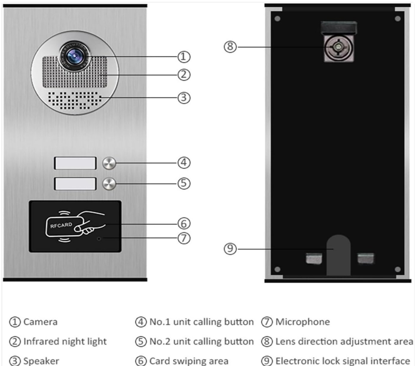
Figure 2: Detailed view of the outdoor unit with labeled components.
