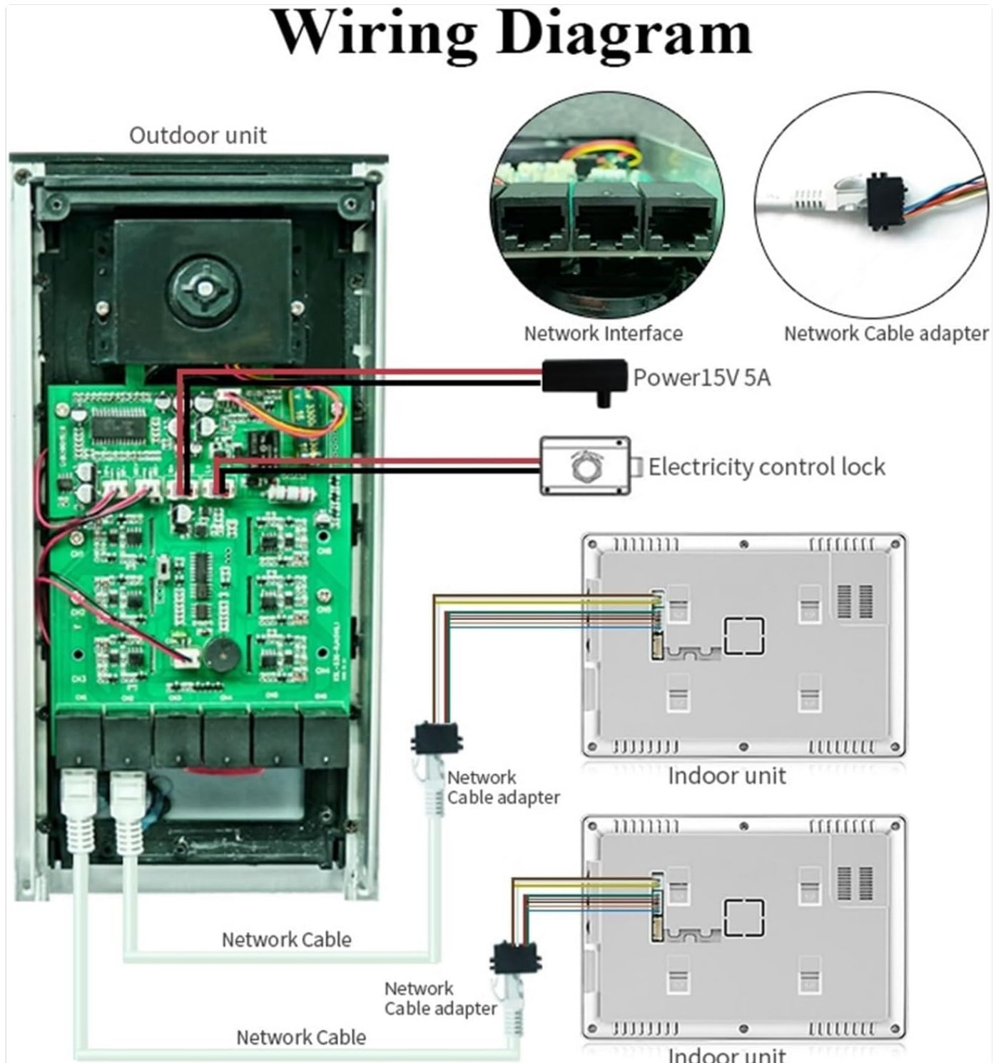
Figure 4: System wiring diagram.
