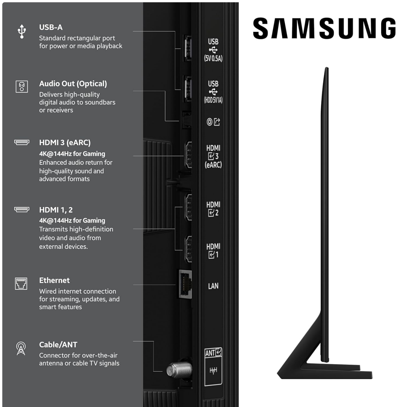
Figure 3.1: Rear view of the TV showing available connection ports.
