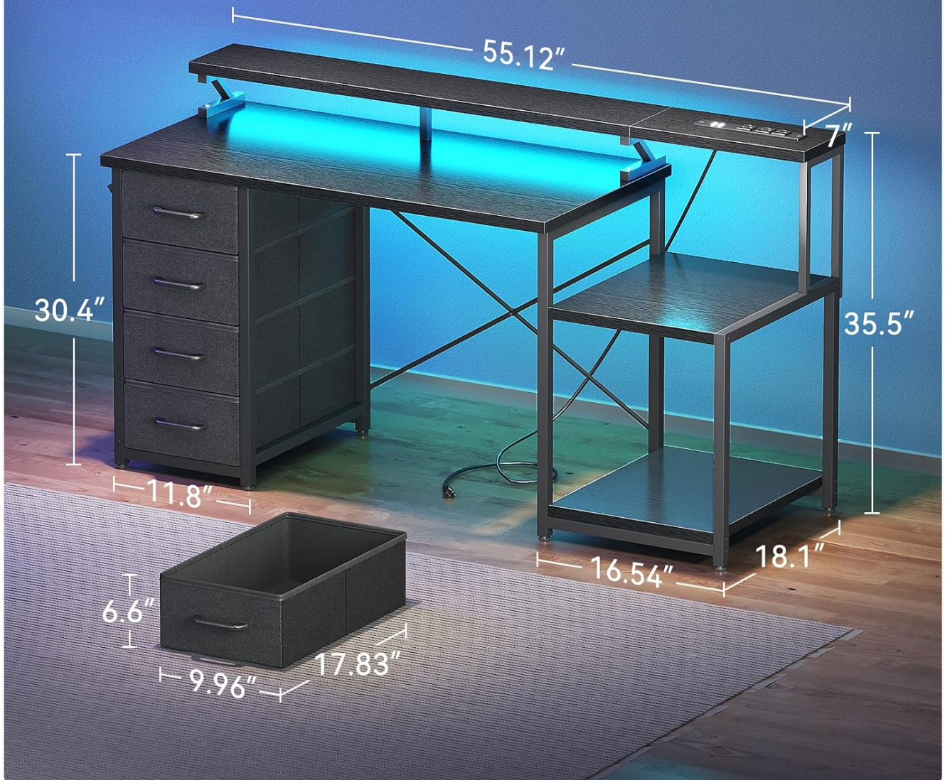
Figure 6: Detailed product dimensions of the ODK desk. This image provides a clear visual breakdown of the desk's height, width, depth, and individual component measurements, including the monitor stand and drawers.
