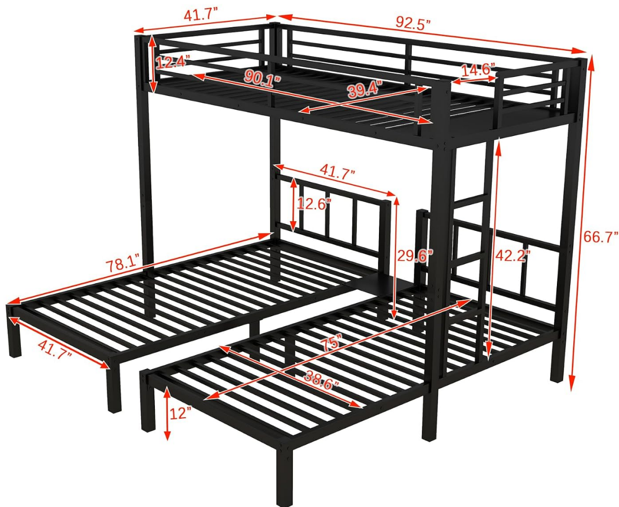
Image: A diagram illustrating the detailed dimensions of the Bellemave Triple Bunk Bed in inches.
