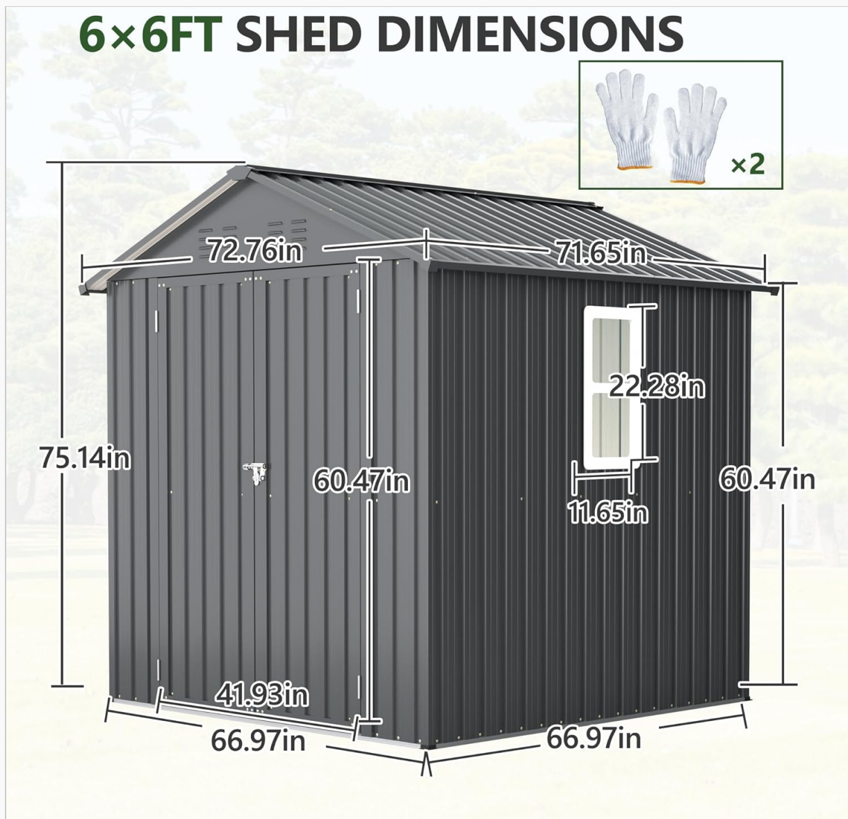
Image: Dimensions of the 6x6ft Outdoor Storage Shed.
