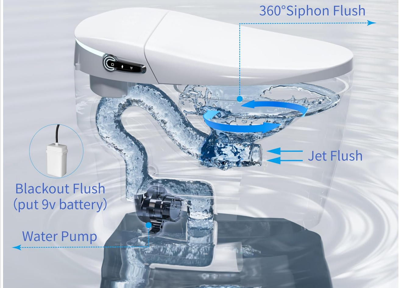
Figure 6.4: Internal view of the double pump assisted flushing system.
