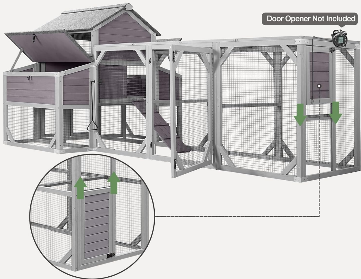
Image 4.1: Detail of the sliding door designed for an automatic door opener (not included).
