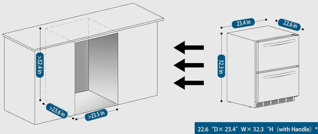
Image 3.1: A diagram illustrating the flexibility of the HCK refrigerator for both built-in and freestanding installations, emphasizing the front ventilation design.
