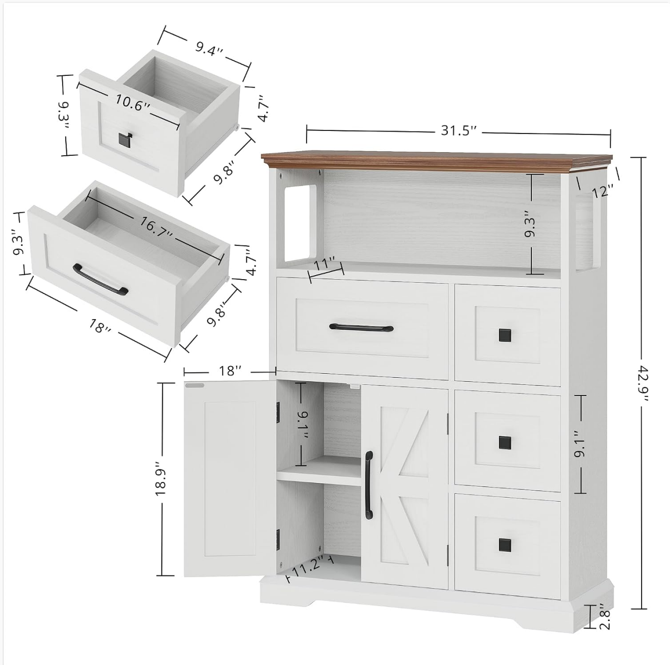
Image 4.1: Dimensional diagram for assembly reference.
