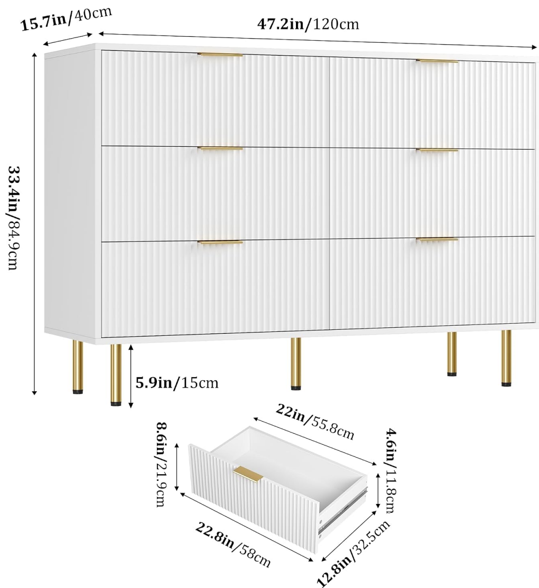
Image 8.1: A detailed diagram illustrating the overall dimensions of the dresser and individual drawer dimensions.
