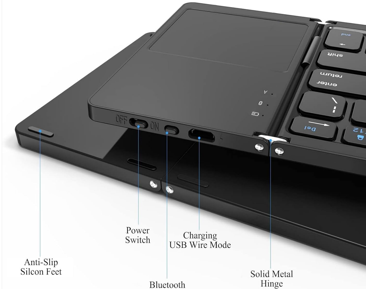
Image 4.1: Key features on the side of the keyboard, including the power switch and charging port.
