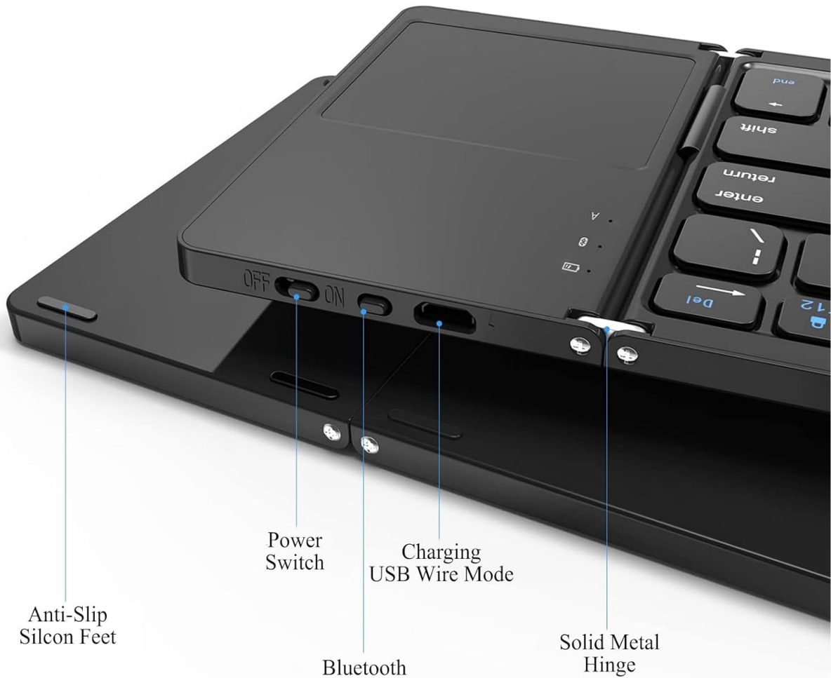
Image: Key components of the keyboard including power switch and charging port.
