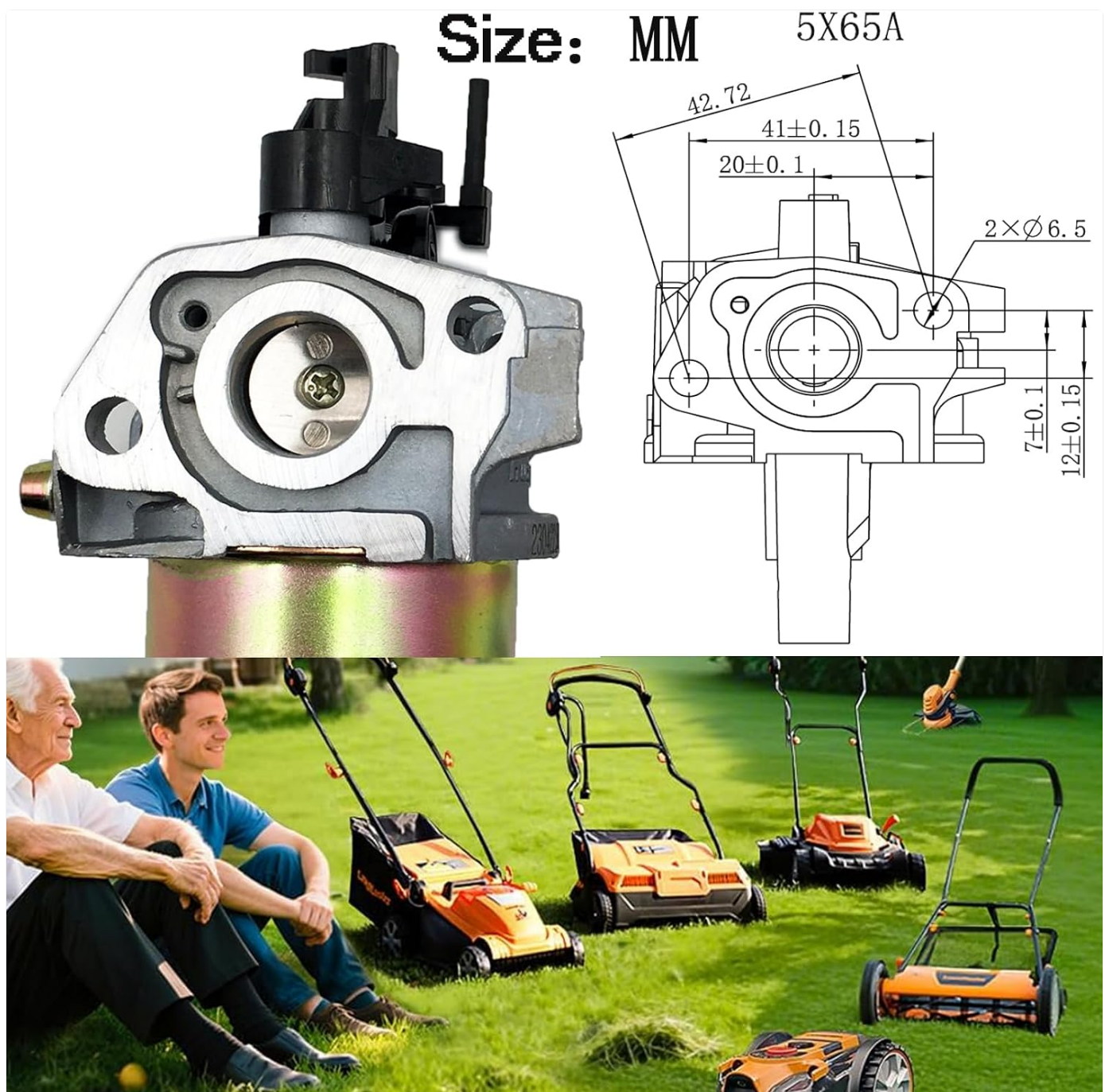
Image 8.1: Technical diagram illustrating key dimensions and specifications of the carburetor.
