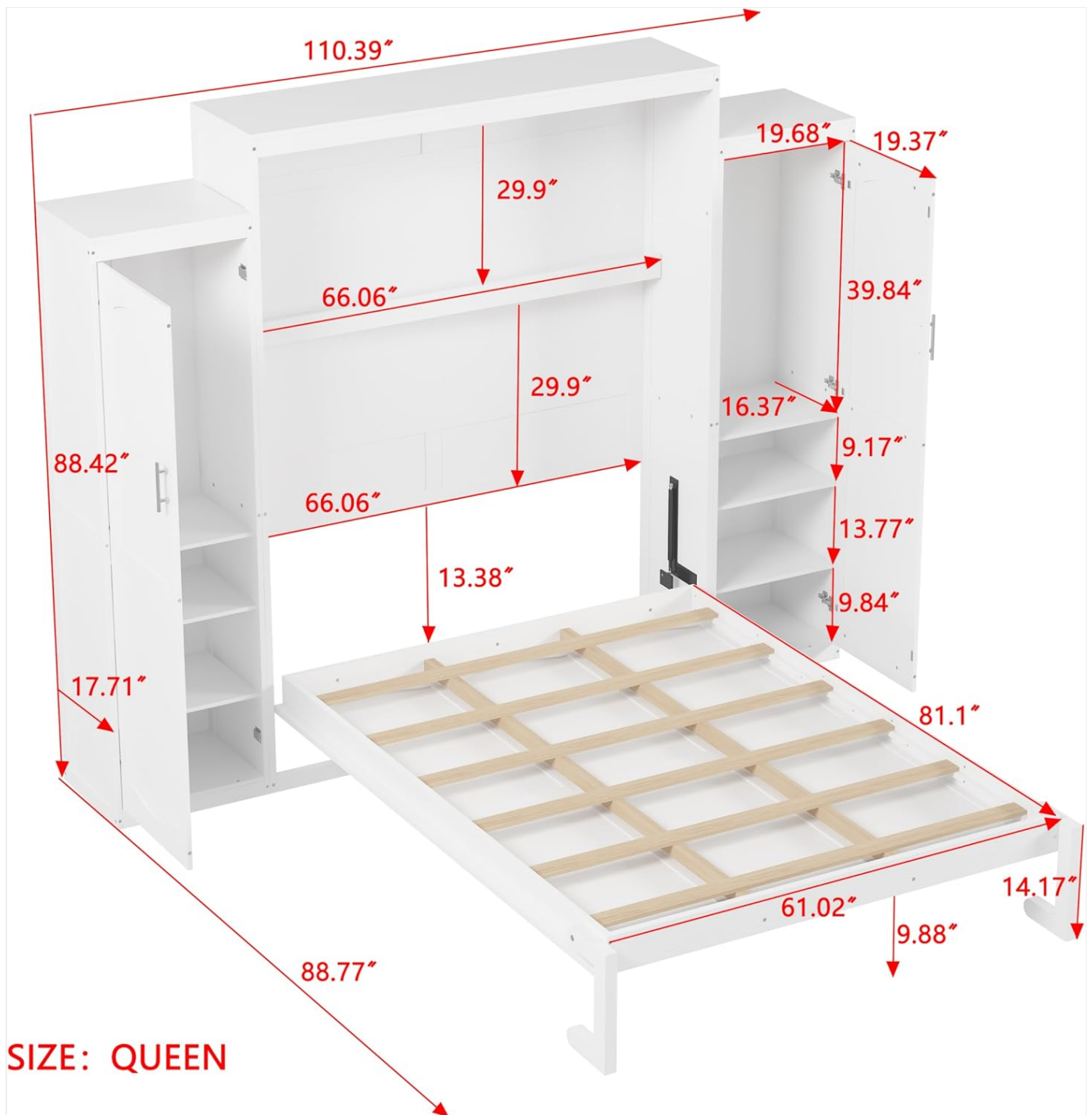
Image: Detailed dimensions of the DERCASS Queen Murphy Bed, showing overall length, width, height, and internal measurements of the bed frame, wardrobes, and storage shelf. The bed measures 88.77 inches in length, 110.39 inches in width (including wardrobes), and 88.42 inches in height.
