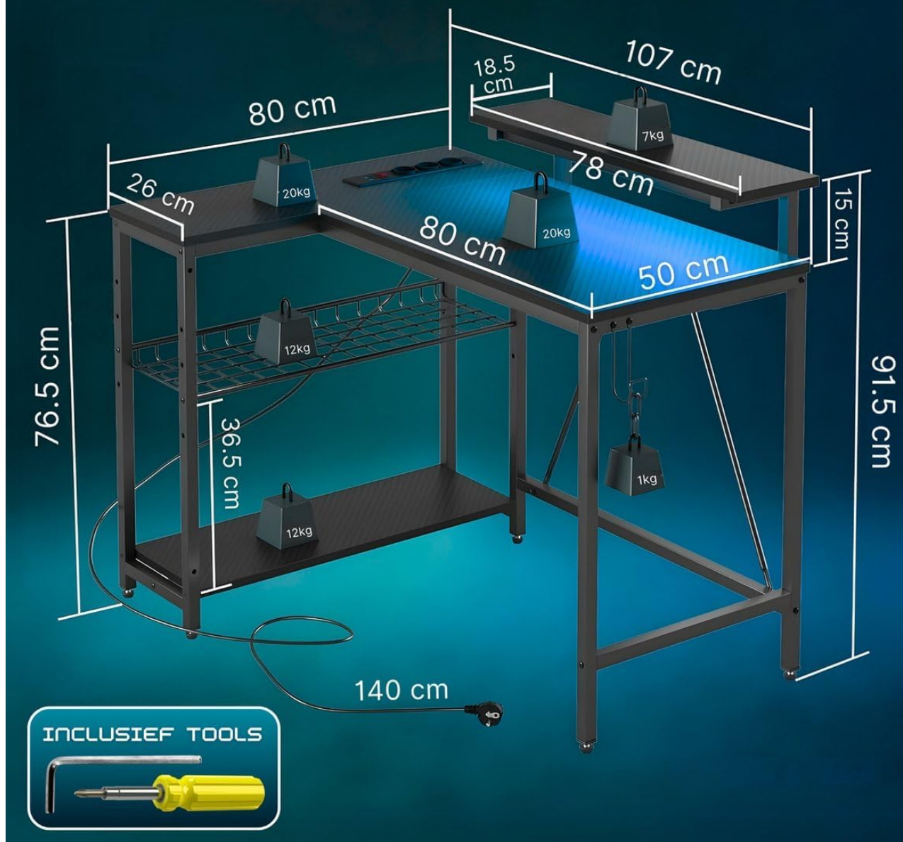
Figure 3.1: Dimensions of the L-shaped gaming desk, illustrating its size and various storage compartments. Tools for assembly are also shown.
