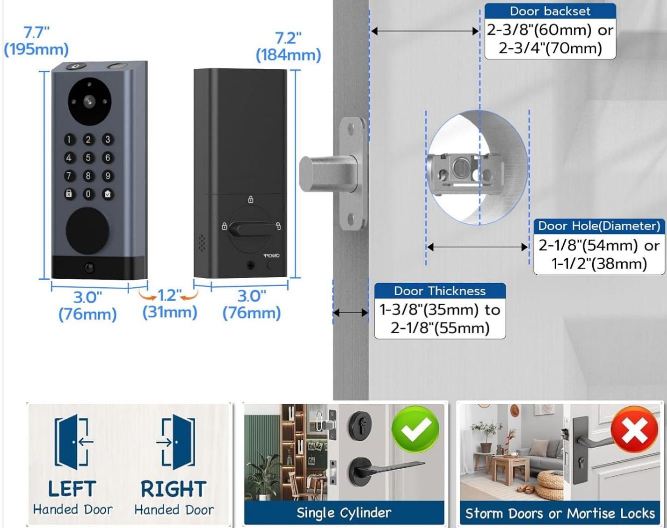
Figure 2: Door Lock Set Dimensions and Compatibility.
