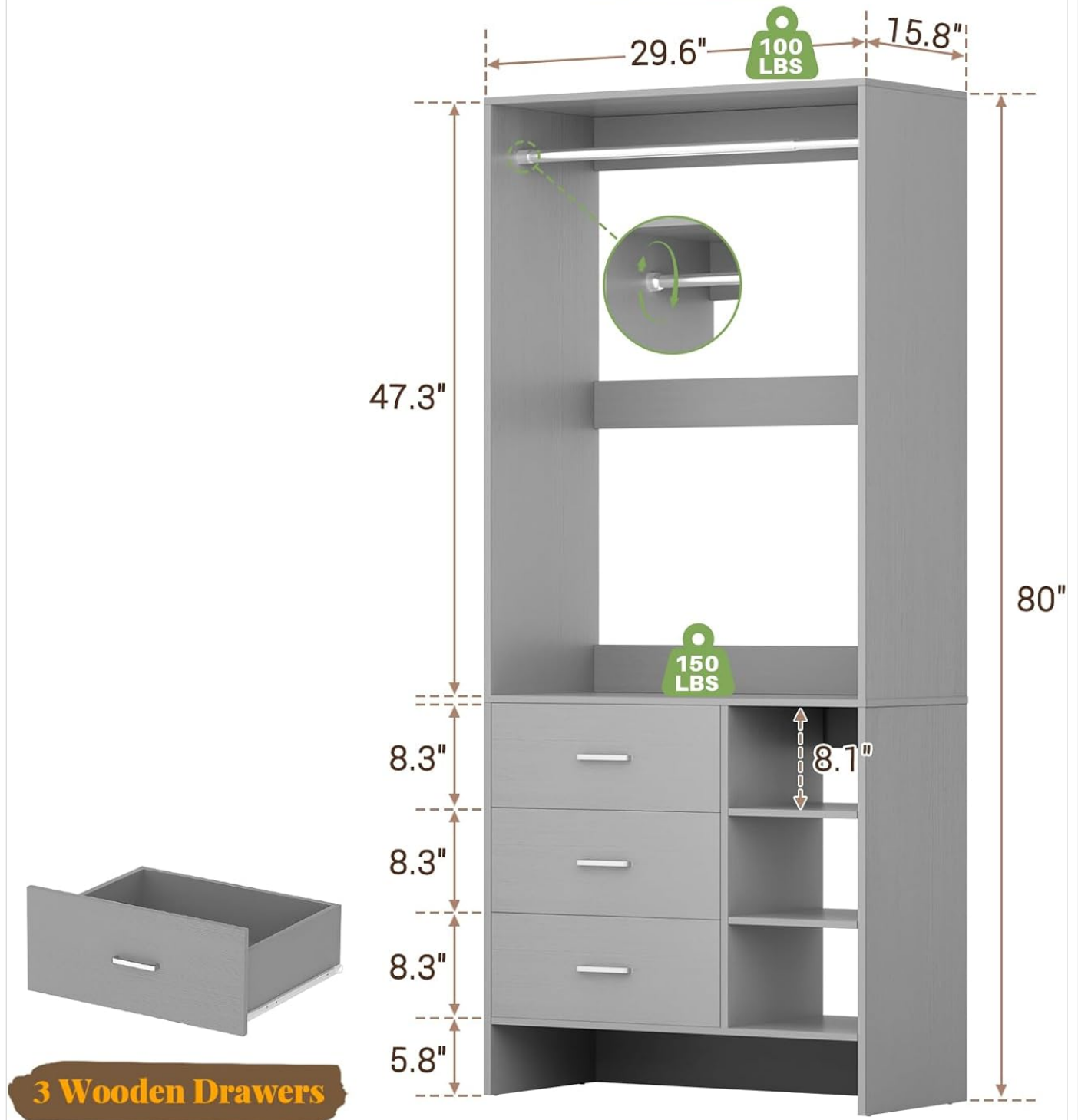
Image 4: Dimensional drawing of the closet system, including measurements for overall size, hanging space, and drawers.
