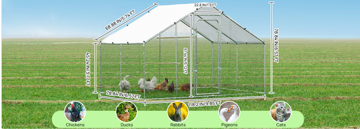
Image 8.1: Detailed dimensions of the chicken coop.
