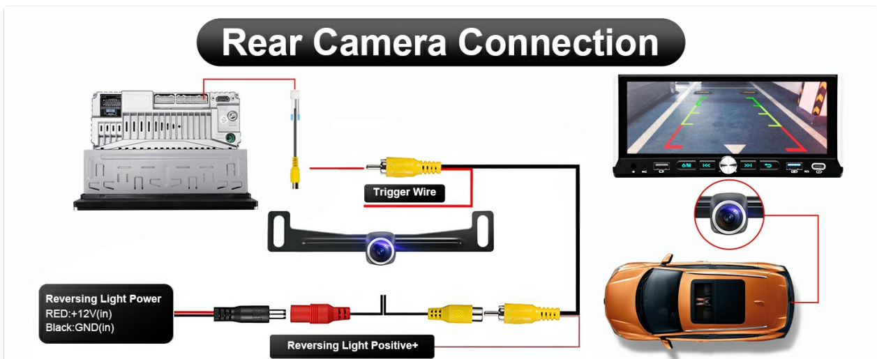
Image 4.2: Rear camera connection diagram.
