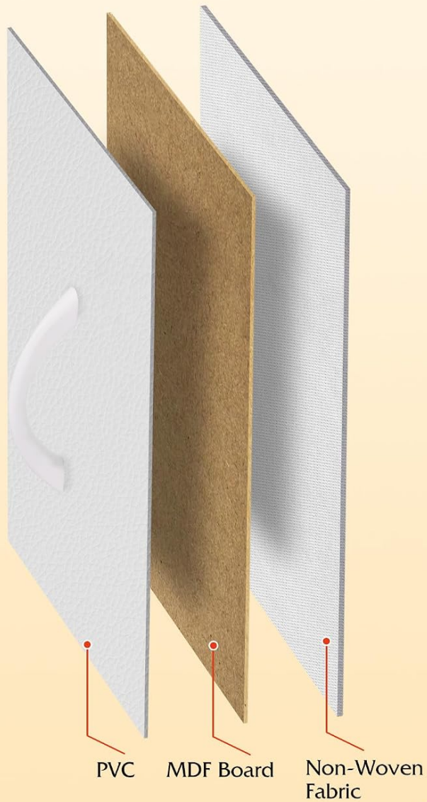
Figure 3.6: Diagram illustrating the three-layer construction of the fabric drawers: PVC, MDF Board, and Non-Woven Fabric, emphasizing durability, breathability, and ease of handling.
