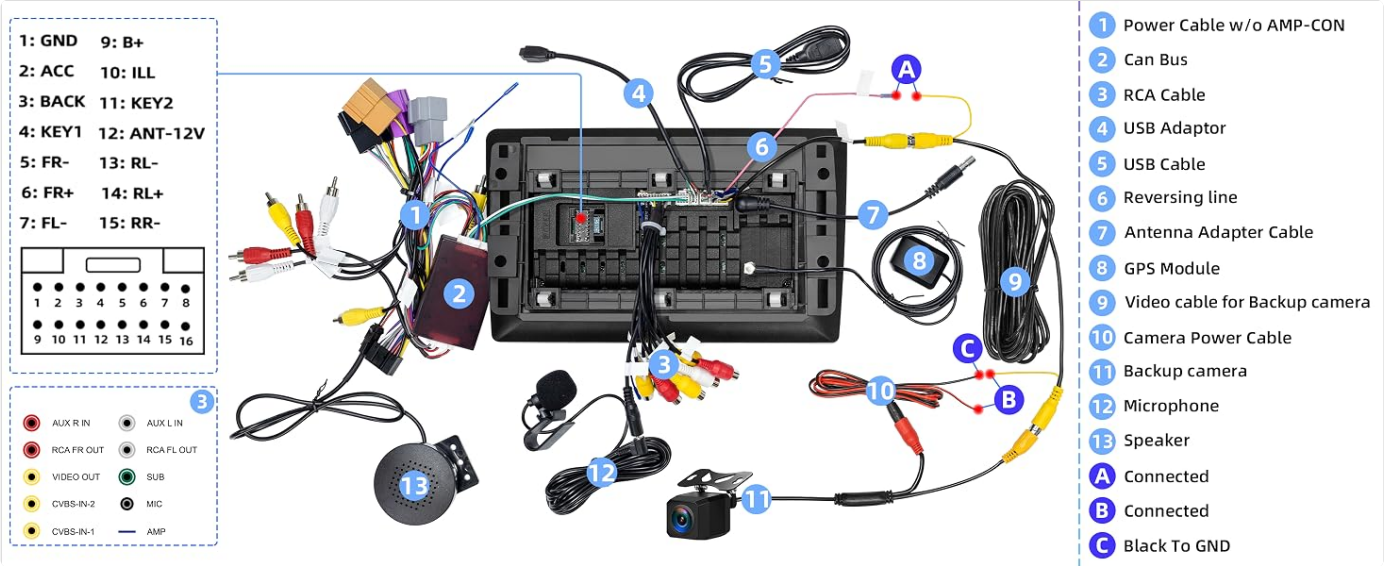
Figure 3: Wiring Diagram. This diagram illustrates the various input and output connections on the back of the head unit, including power, speaker outputs, RCA cables, USB, GPS, and camera inputs.
