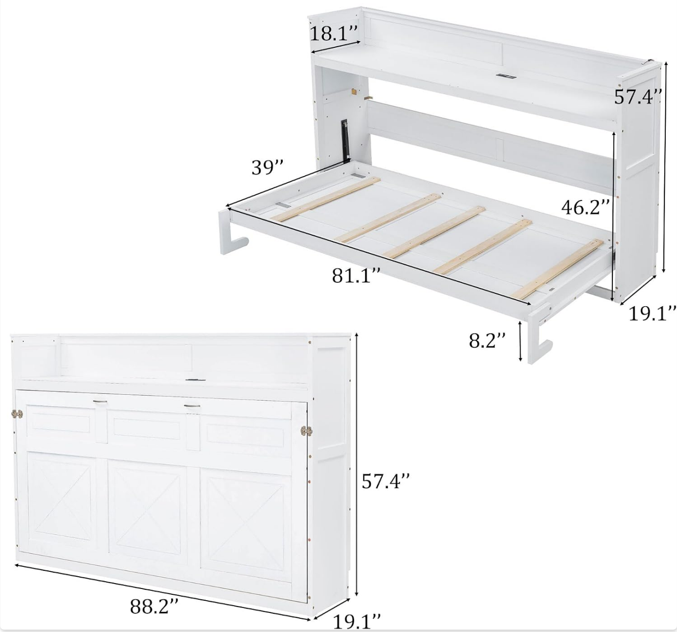
Figure 7: Detailed dimensions of the Murphy Bed.
