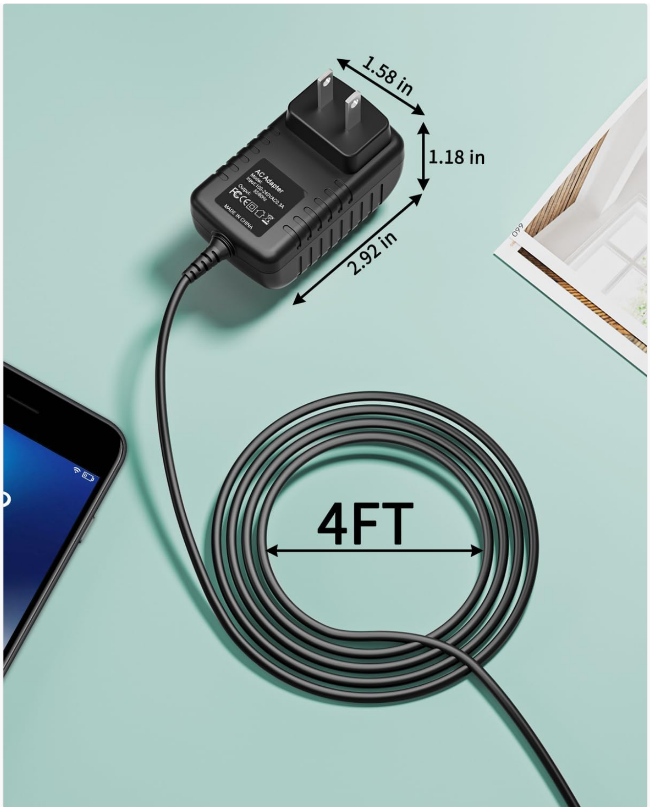
Image: A visual representation of the adapter's dimensions (approximately 2.92 inches long, 1.58 inches wide, 1.18 inches deep) and its 4-foot (4FT) cord length.
