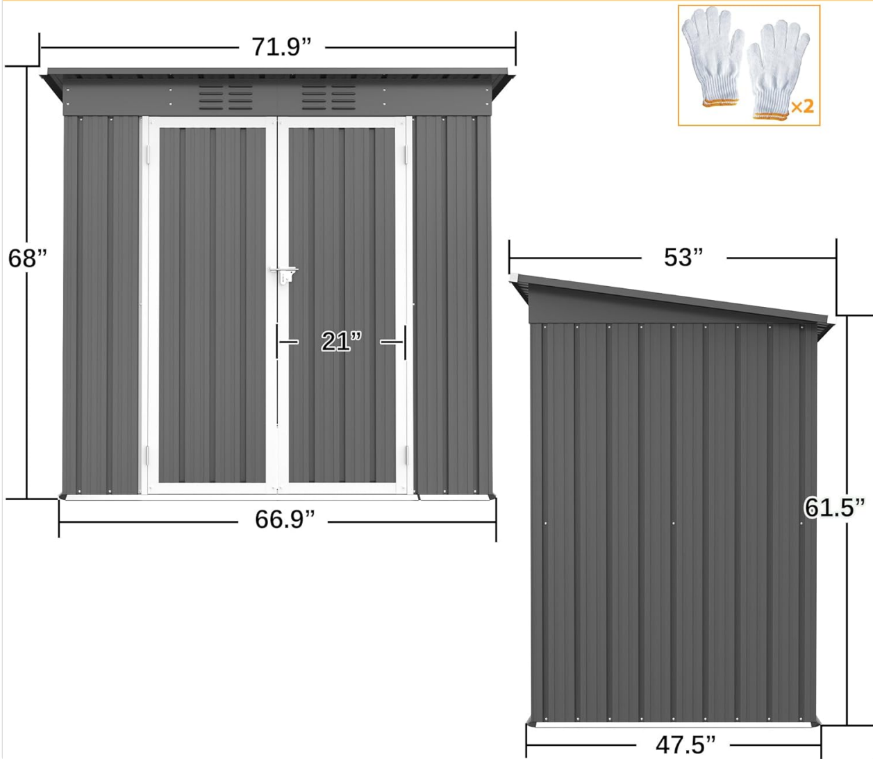
Image: Front and side view with key dimensions of the shed.
