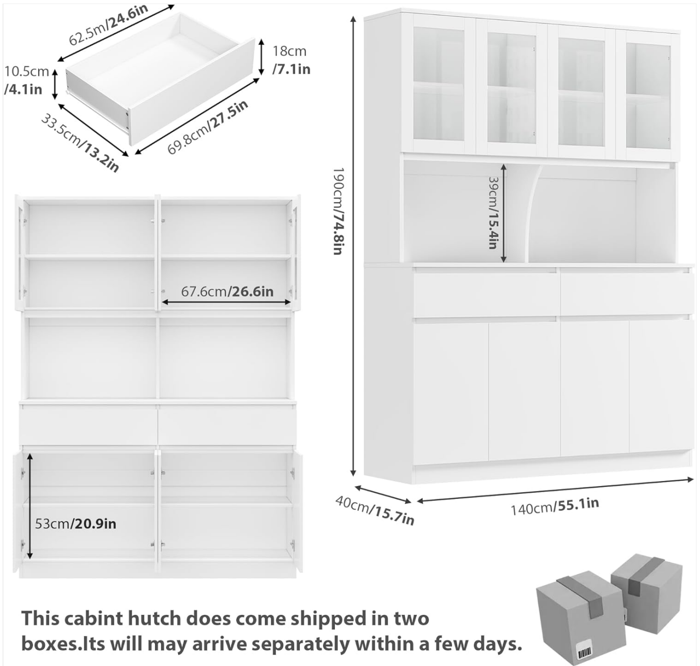
Image 1: Overall dimensions and component breakdown of the cabinet.
