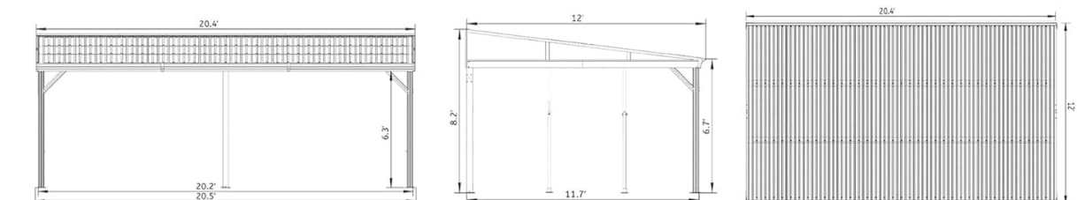
Image: A detailed diagram illustrating the overall dimensions of the 12' x 20' wall-mounted hardtop gazebo, including height, length, and width measurements.
