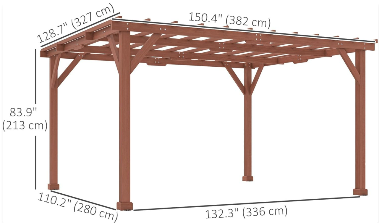
Figure 6: Detailed dimensions of the Outsunny Wood Pergola.
