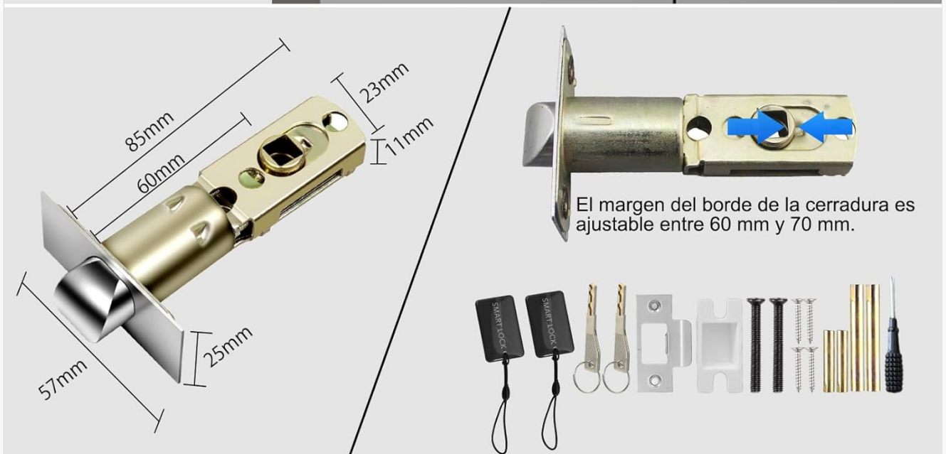
Figure 5: Latch Backset Adjustment
