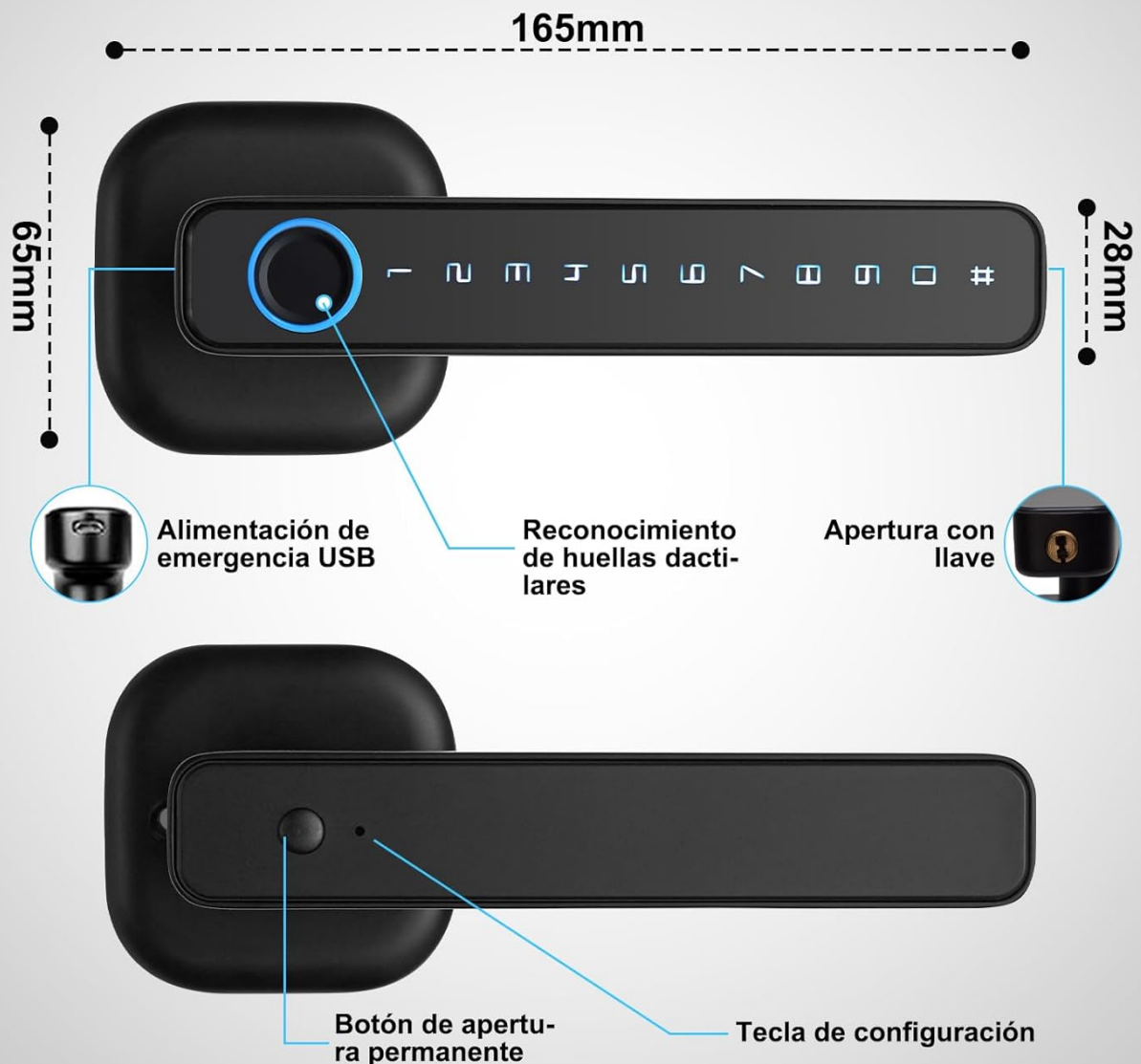
Figure 3: Product Dimensions and Key Components
