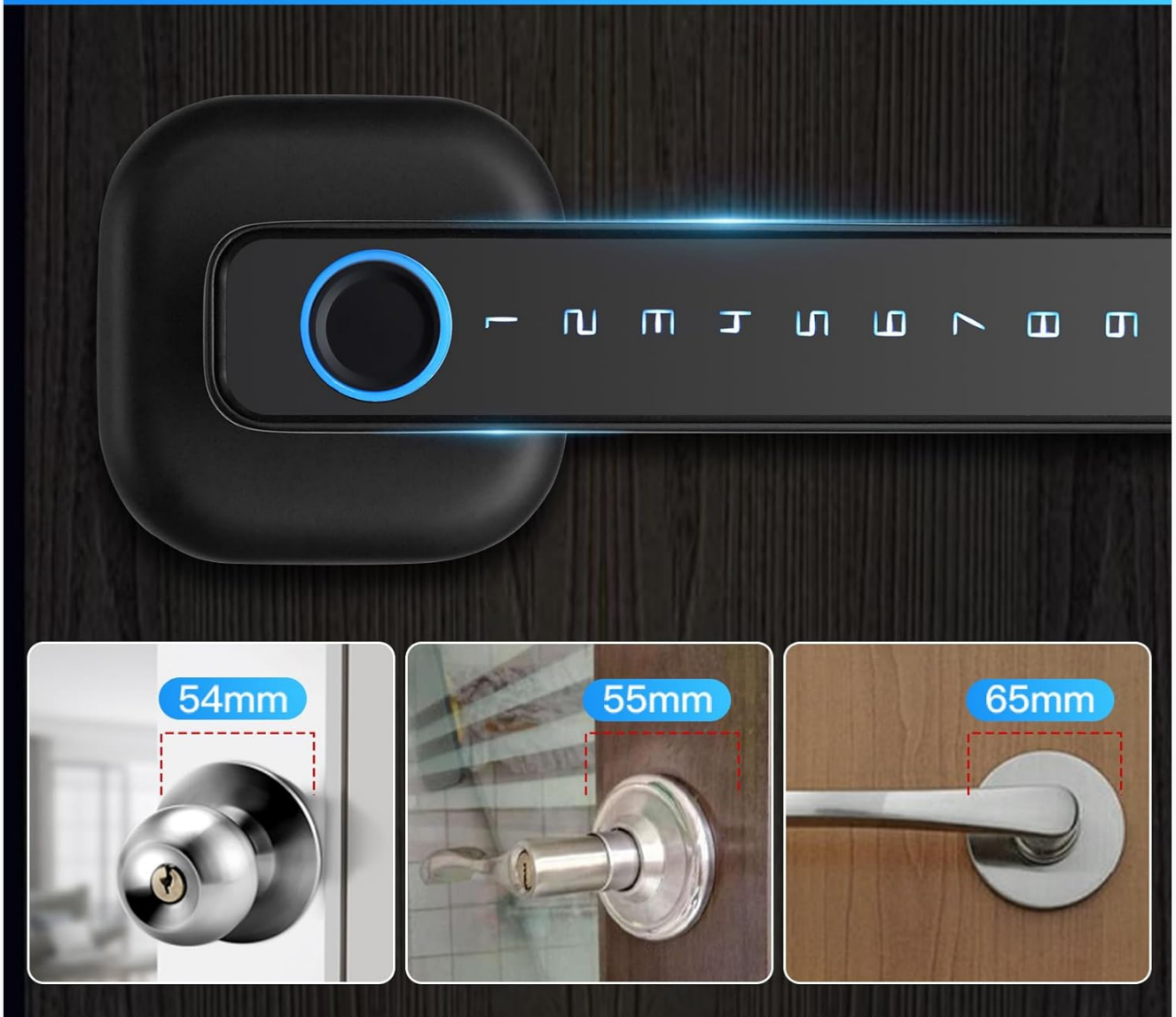
Figure 4: Compatibility with Various Keyhole Types
