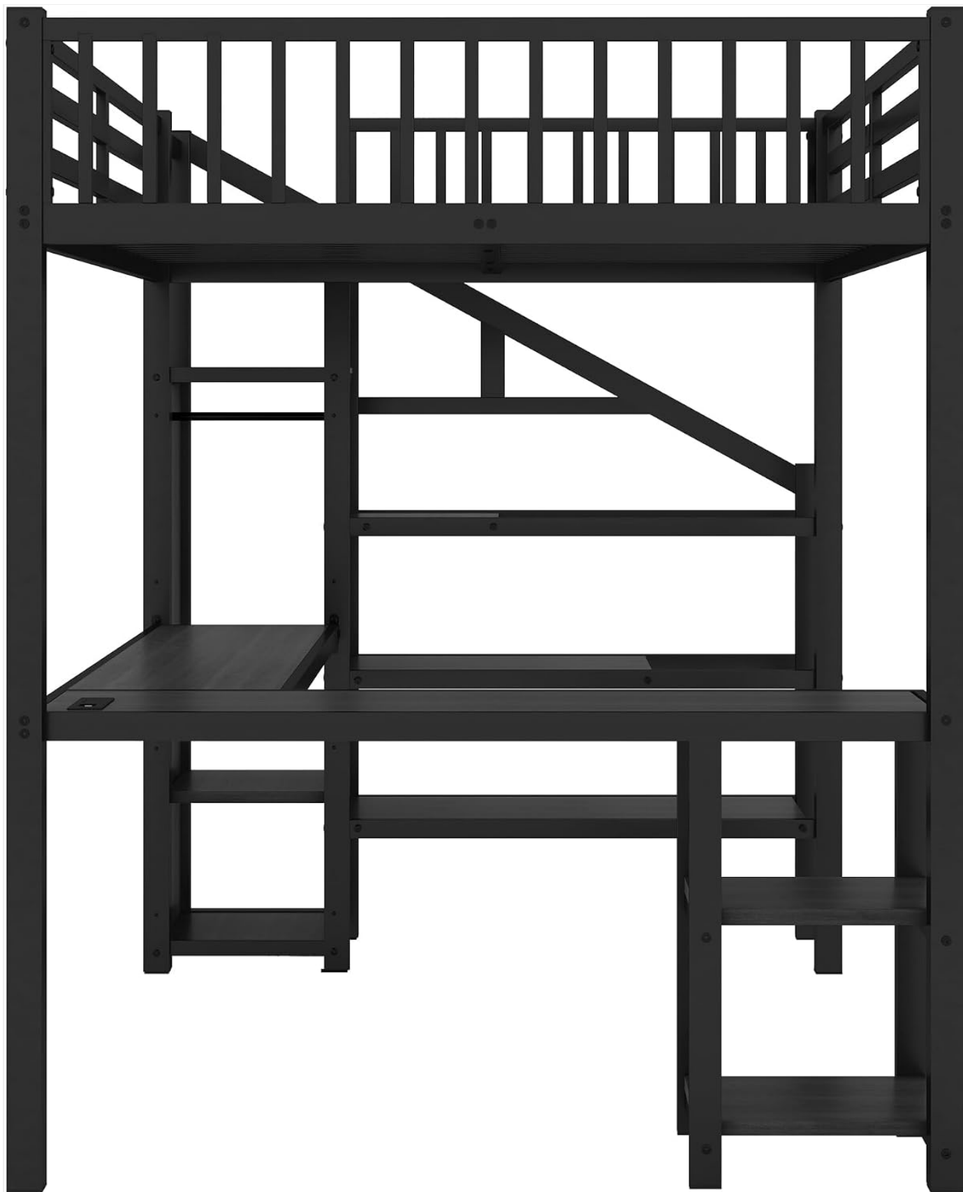
Image 4.2: Front view of the assembled loft bed, highlighting the L-shaped desk and the staircase with its integrated storage cabinet.
