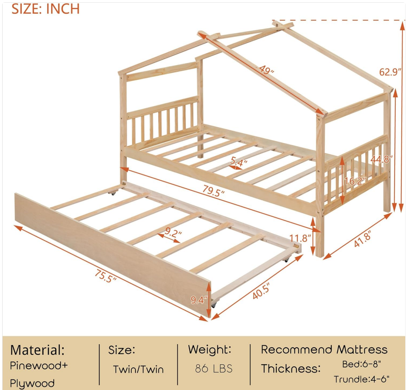
Image 2.1: Technical drawing illustrating the dimensions and material composition of the Twin House Bed with Trundle.
