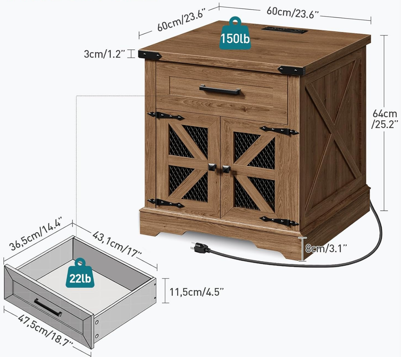
Image 3.1: Product dimensions and weight capacities for the end table and drawer.
