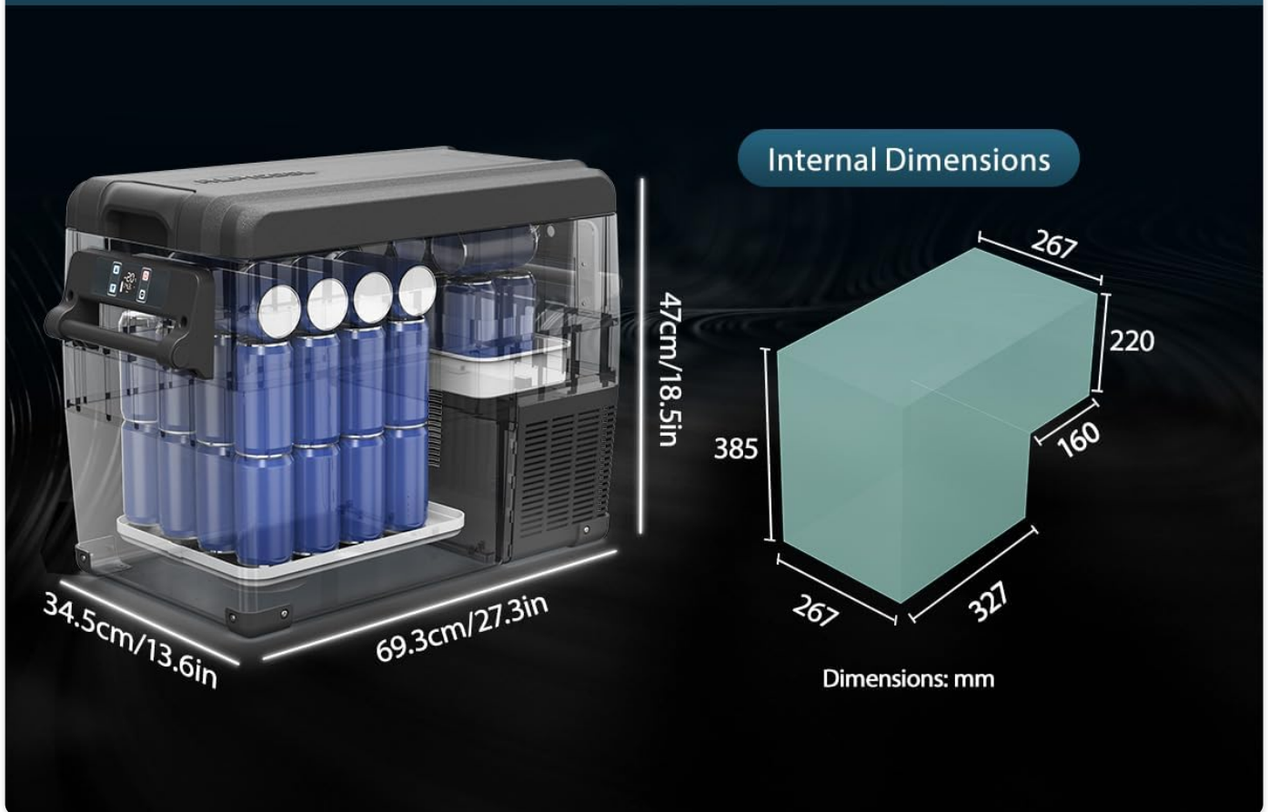
Image 6.1: Diagram showing the 42QT/40L capacity and external/internal dimensions of the Alpicool NCF45.
