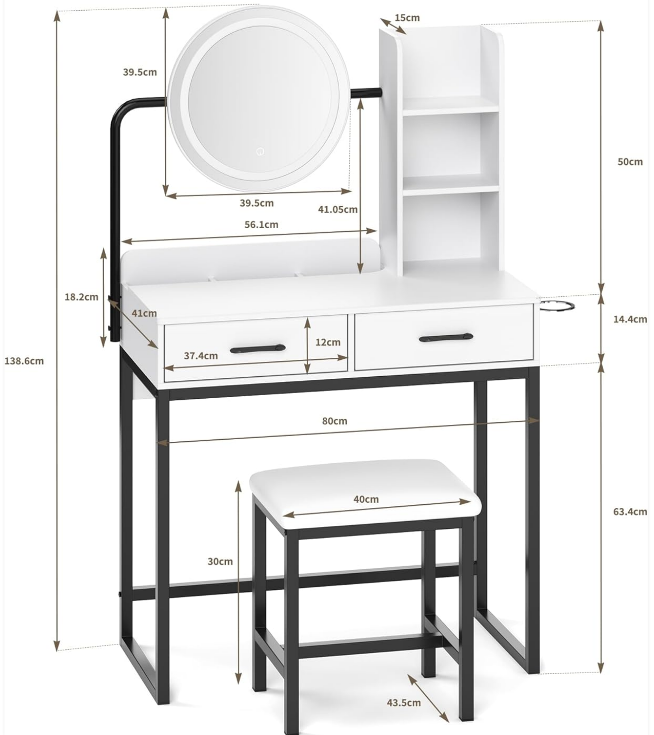
Image 7.1: Detailed dimensions of the vanity desk and stool in centimeters.
