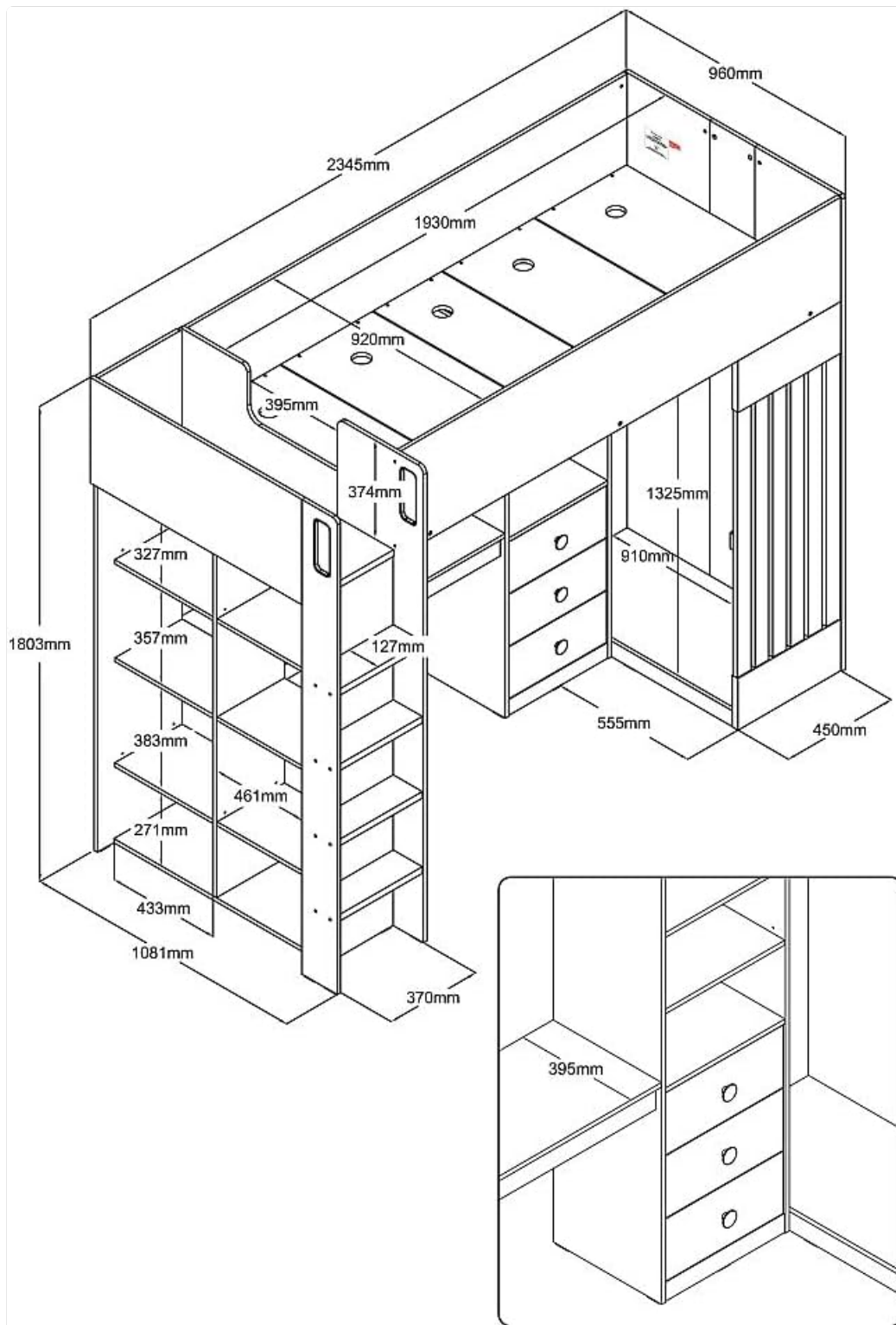
Figure 4: Technical drawing illustrating the dimensions and layout of the LORINTI Loft Bed components.
