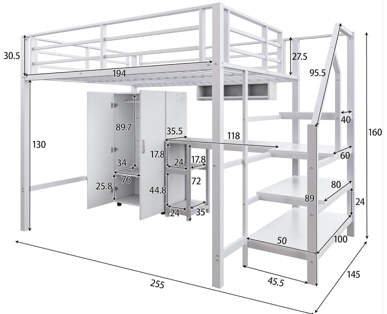
Figure 5.1: The loft bed configured with its desk, wardrobe, and shelving units, demonstrating its practical use.
